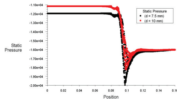
Fig. 9. Effect of throat holes diameter on pressure loss along the x direction
